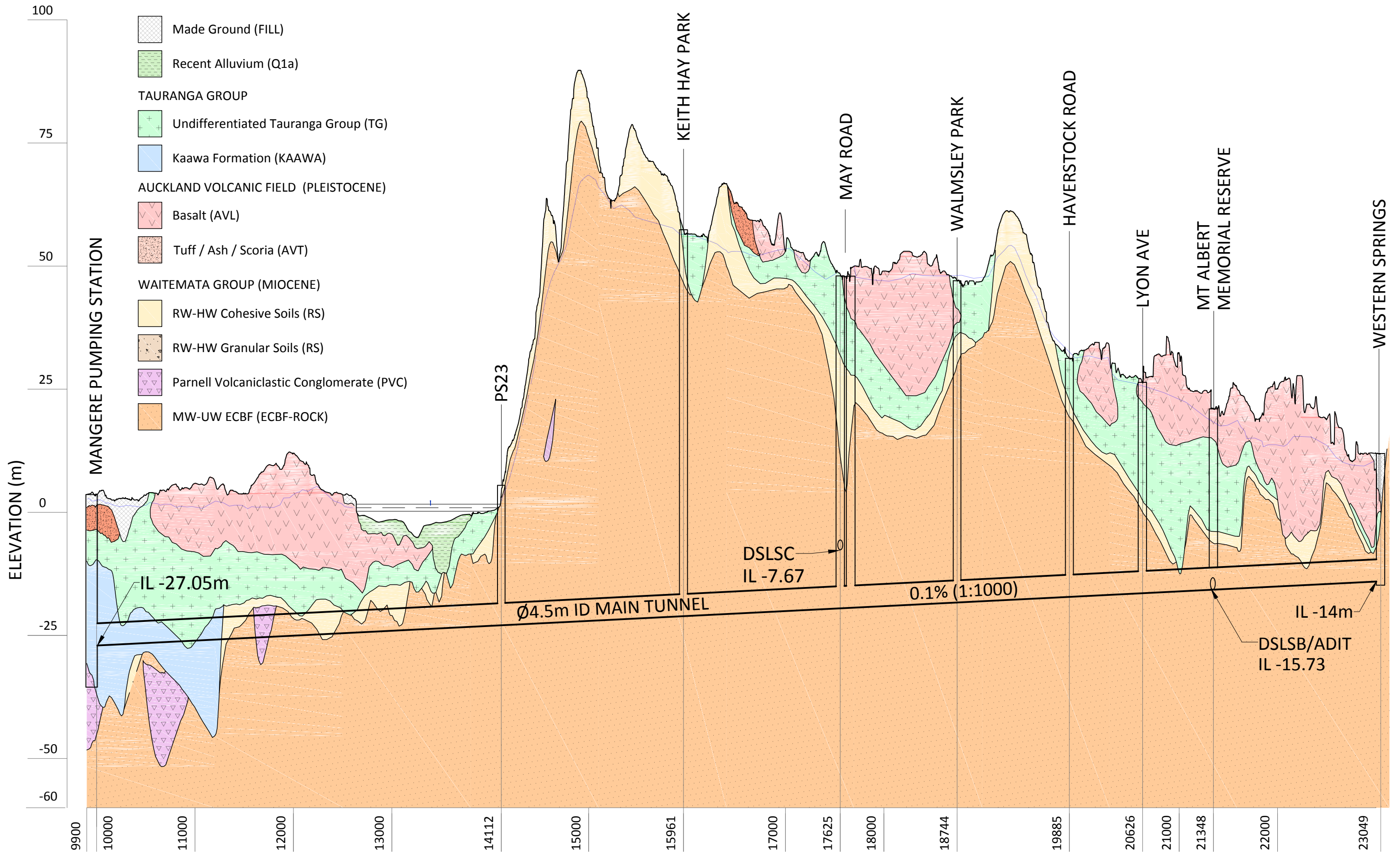
TUNNEL PROFILE NOT TO SCALE
